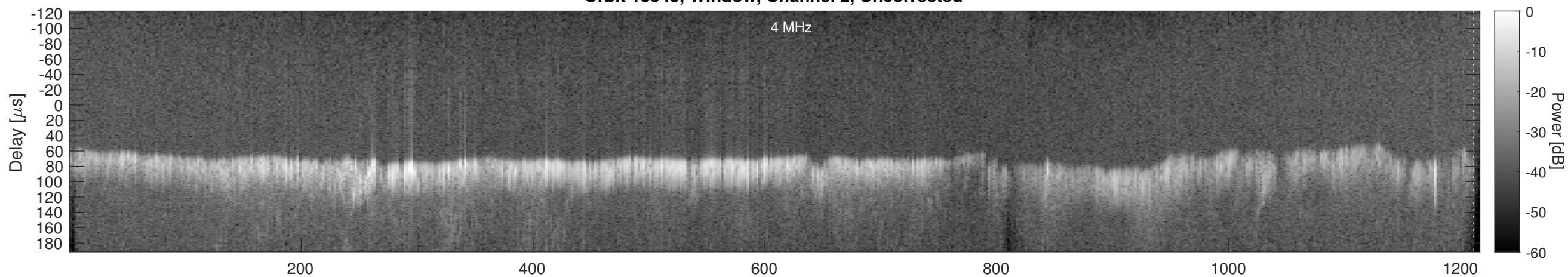
Orbit 13543, Window, Channel 2, Chapman
