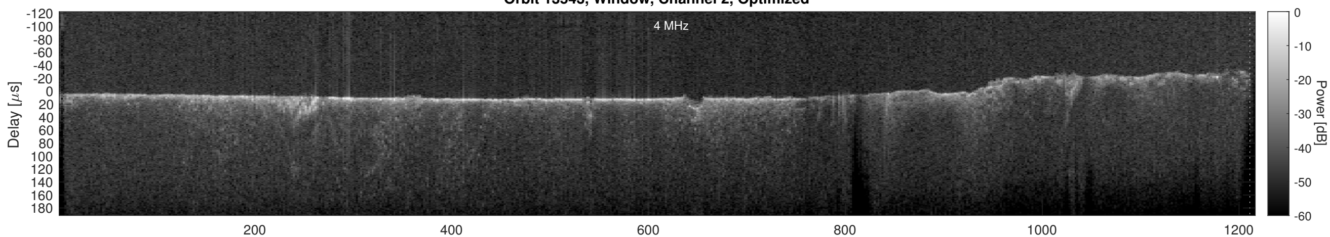
Orbit 13543, Cluttergram
