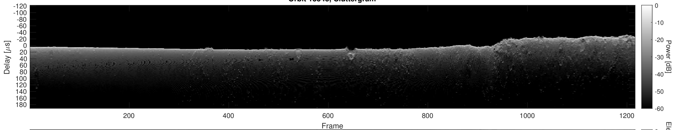
Orbit 13543, Cluttergram
