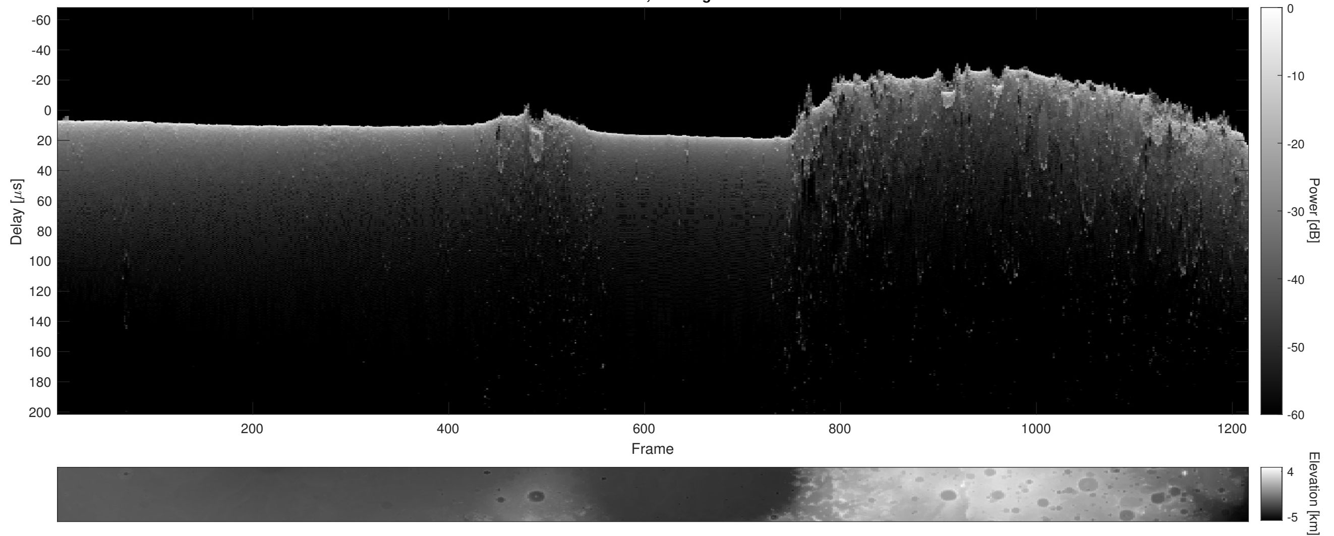
Orbit 13544, Cluttergram
