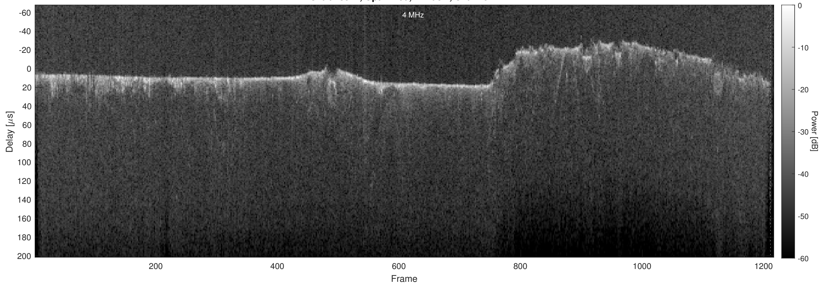
Orbit 13544, Optimized, Window, Channel 2
