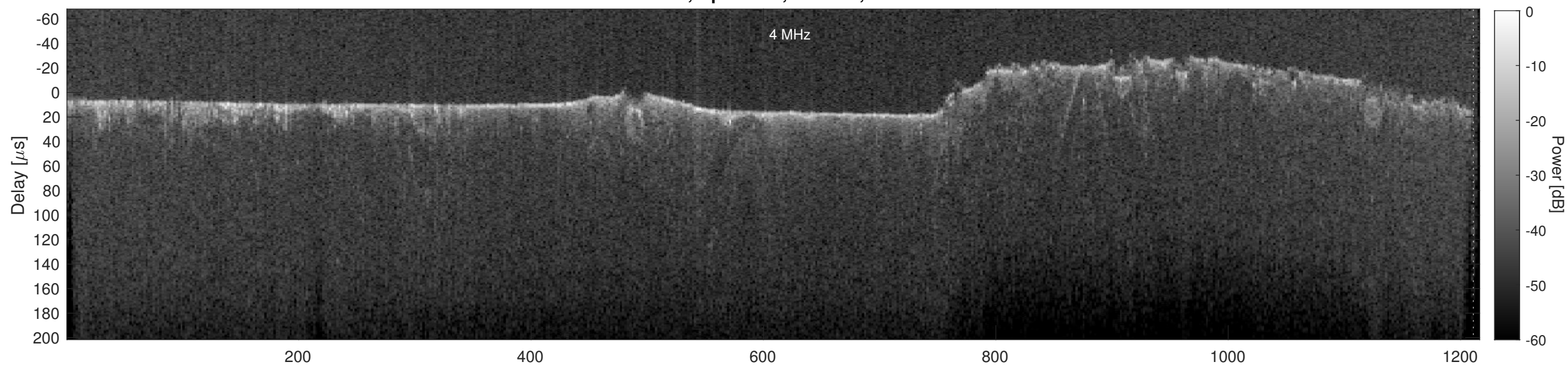
Orbit 13544, Cluttergram
