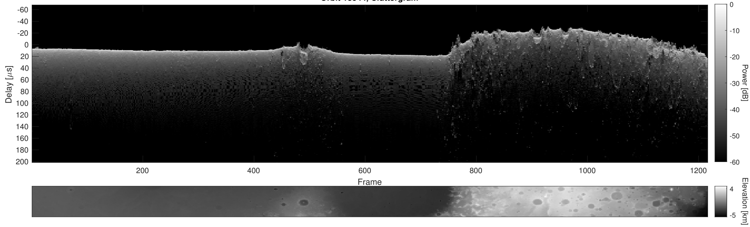
Orbit 13544, Cluttergram
