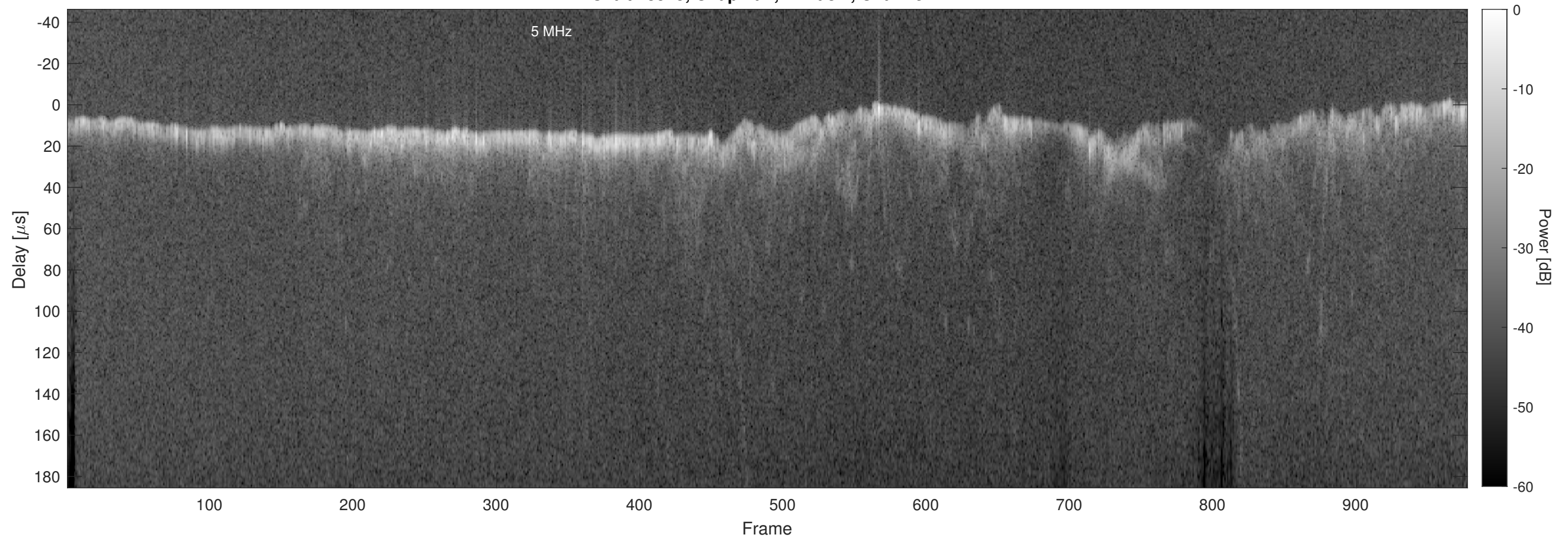
Orbit 13545, Chapman, Window, Channel 2
