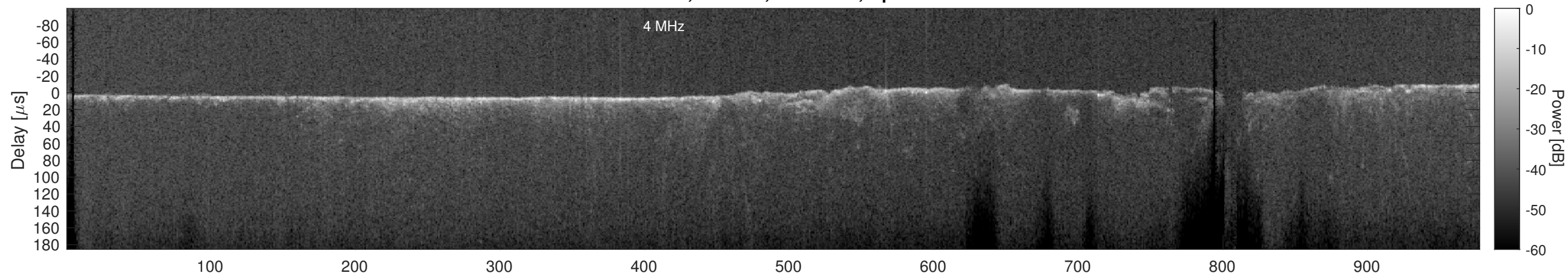
Orbit 13545, Cluttergram
