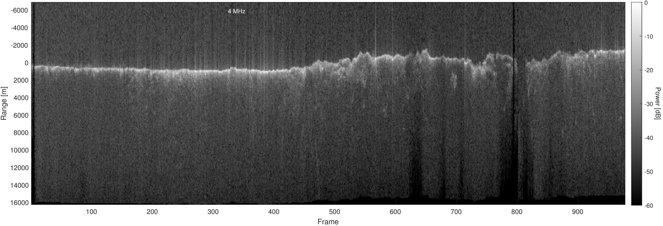
Orbit 13545, Optimized, No Window, Depth-Corrected, Channel 2
