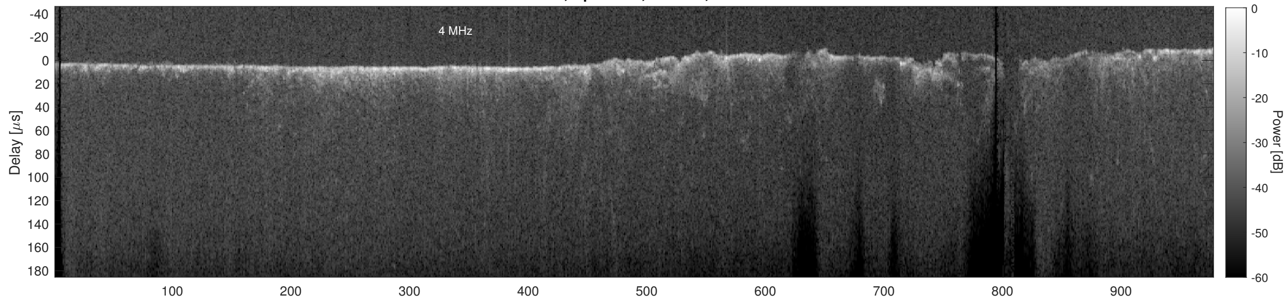
Orbit 13545, Cluttergram
