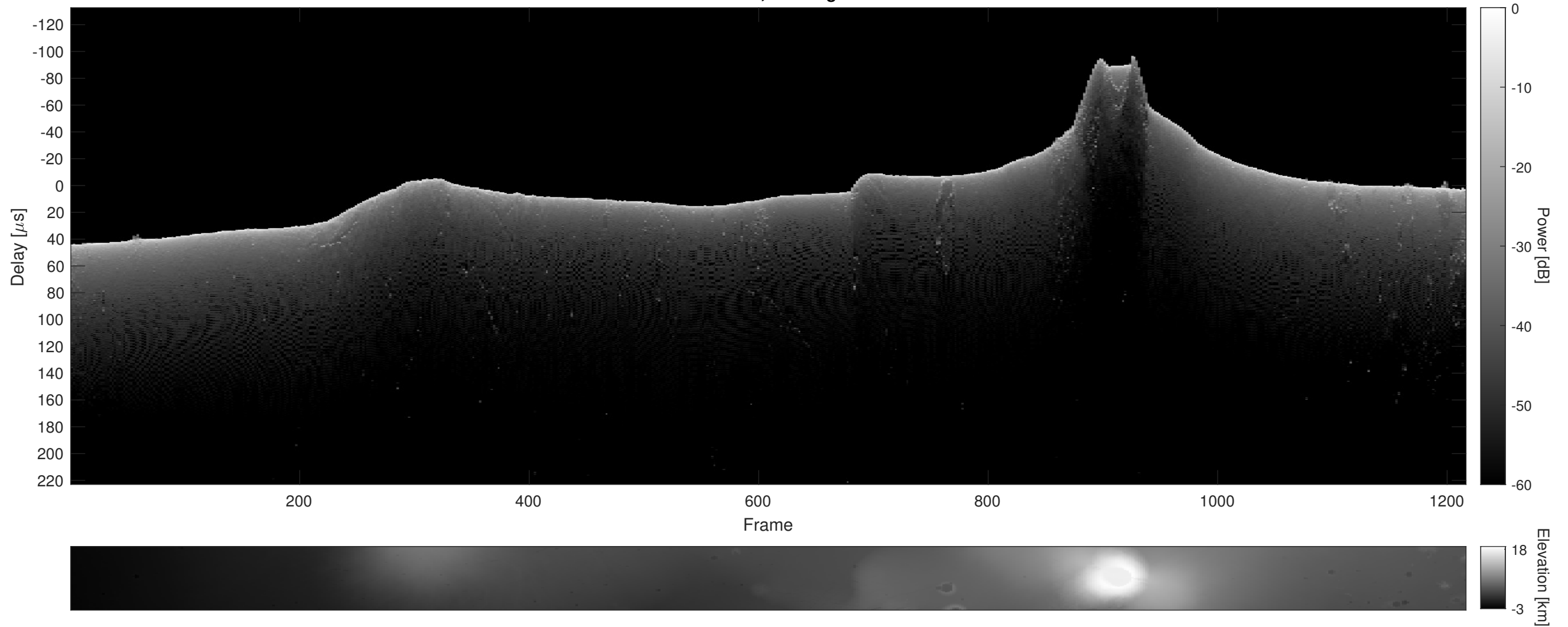
Orbit 13546, Cluttergram
