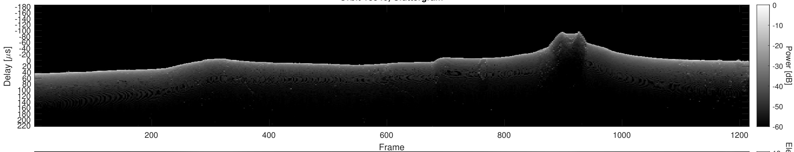
Orbit 13546, Cluttergram
