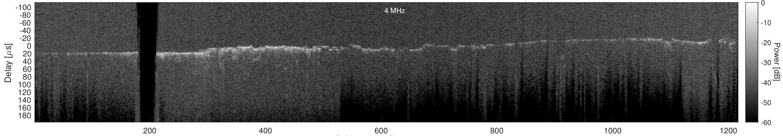
Orbit 13548, Cluttergram
