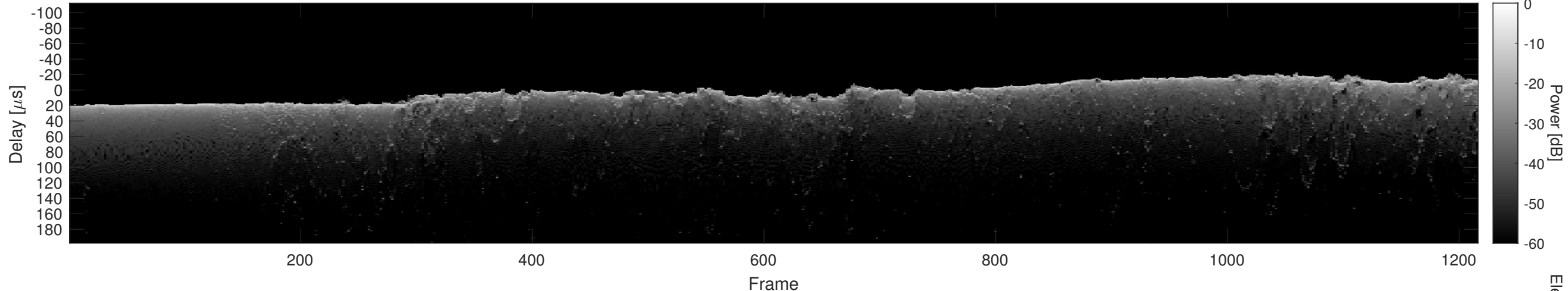
Orbit 13548, Cluttergram
