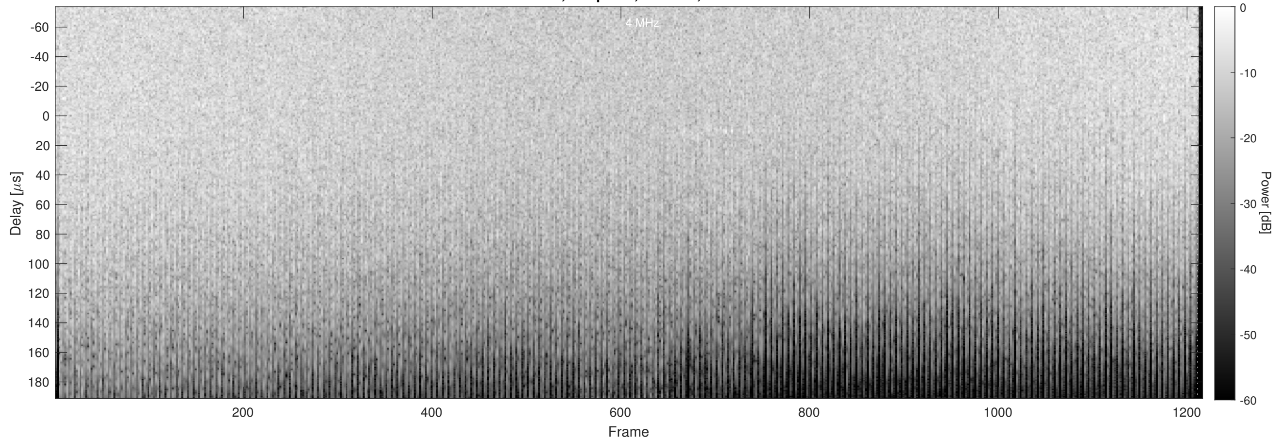
Orbit 13550, Chapman, Window, Channel 2
