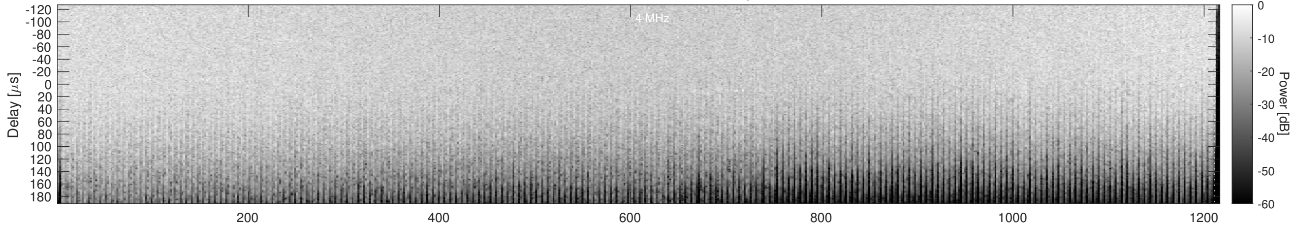
Orbit 13550, Window, Channel 2, Optimized
