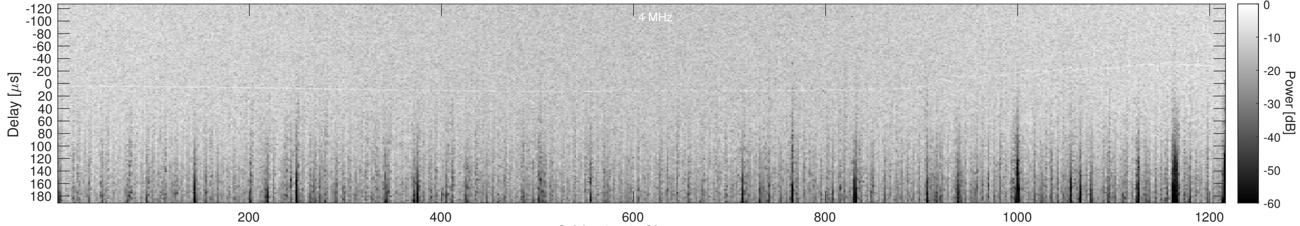
Orbit 13550, Cluttergram
