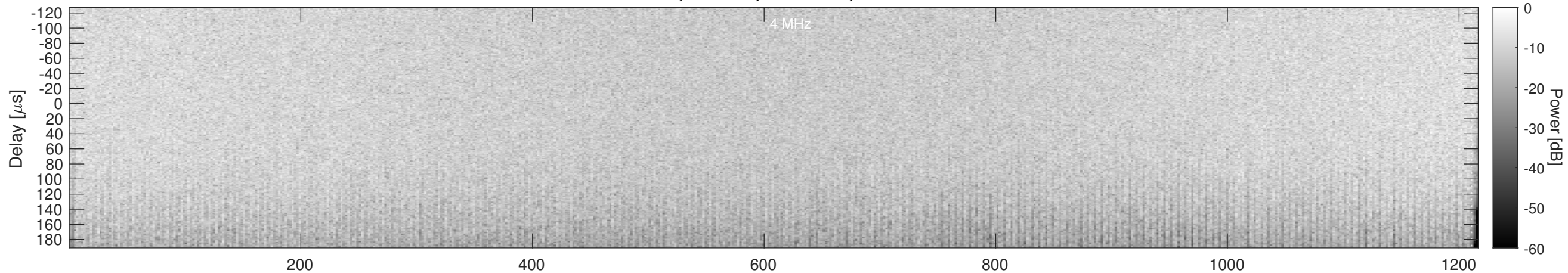
Orbit 13550, Window, Channel 2, Chapman
