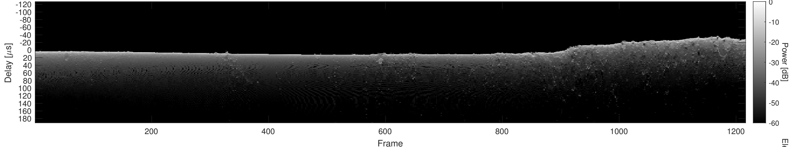
Orbit 13550, Cluttergram
