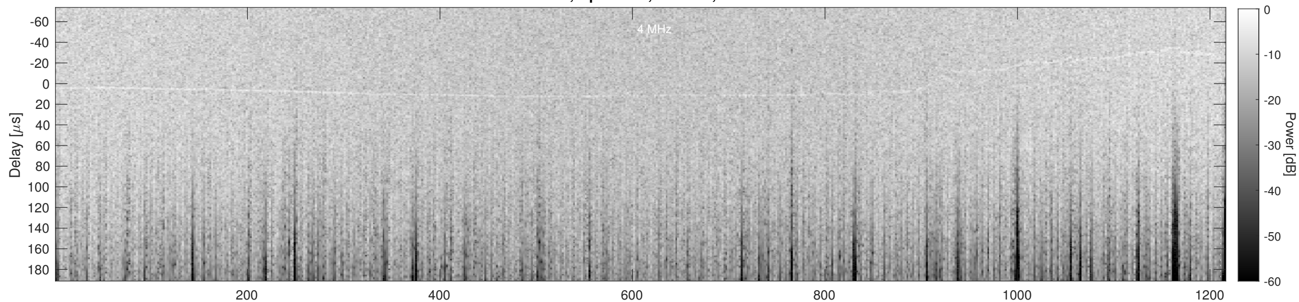
Orbit 13550, Cluttergram
