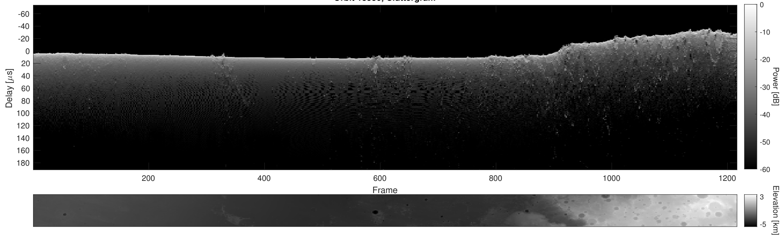
Orbit 13550, Cluttergram
