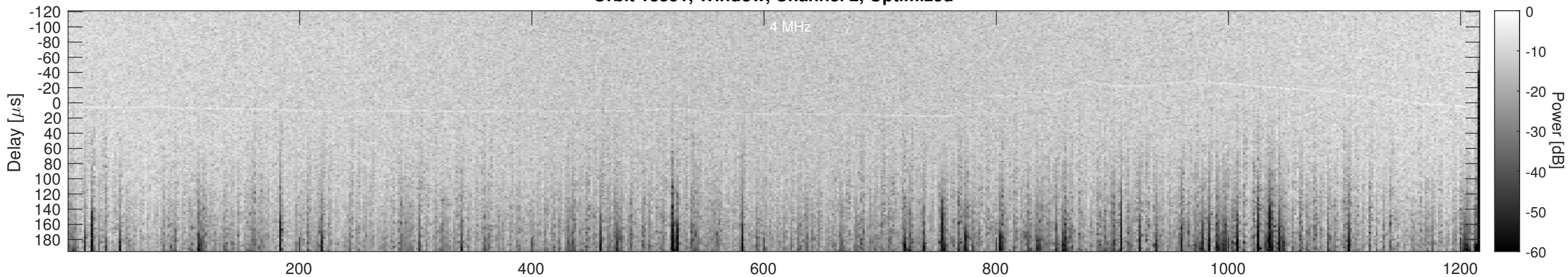
Orbit 13551, Cluttergram
