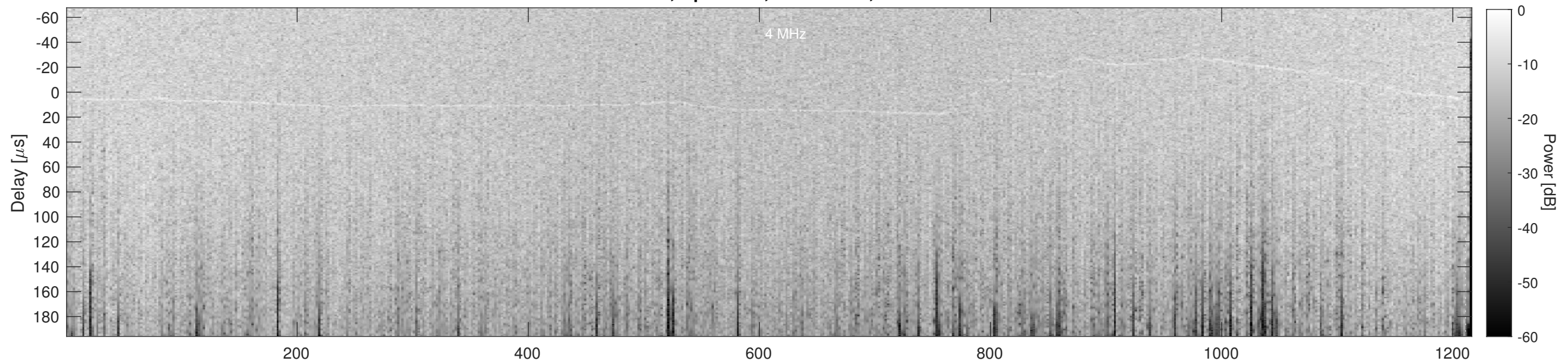
Orbit 13551, Cluttergram
