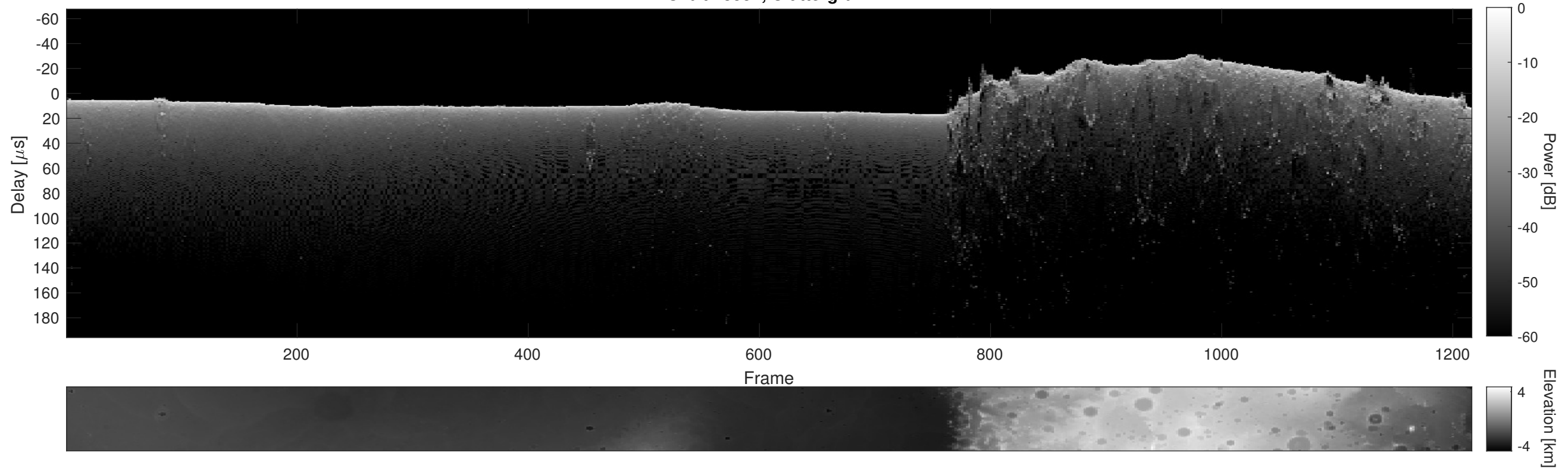
Orbit 13551, Cluttergram
