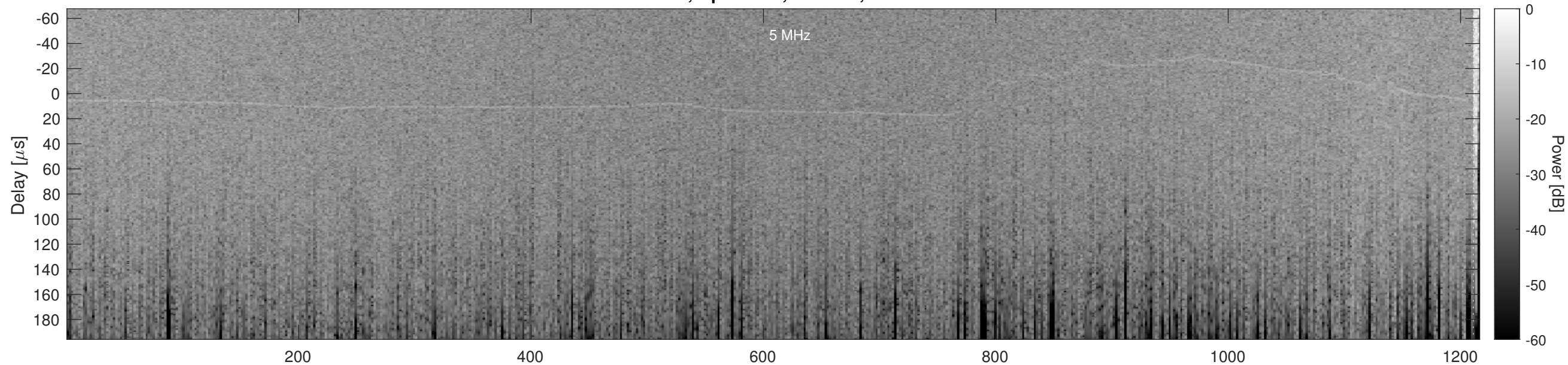
Orbit 13551, Optimized, Window, Channel 2
