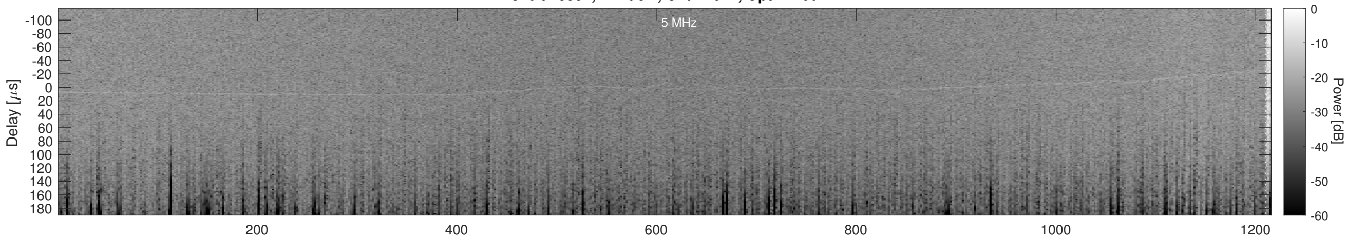
Orbit 13552, Cluttergram
