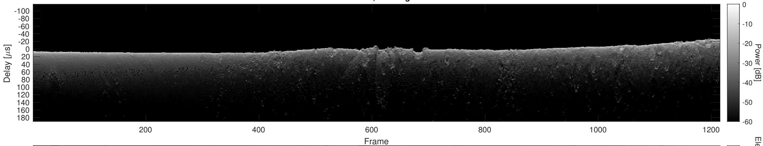
Orbit 13552, Cluttergram
