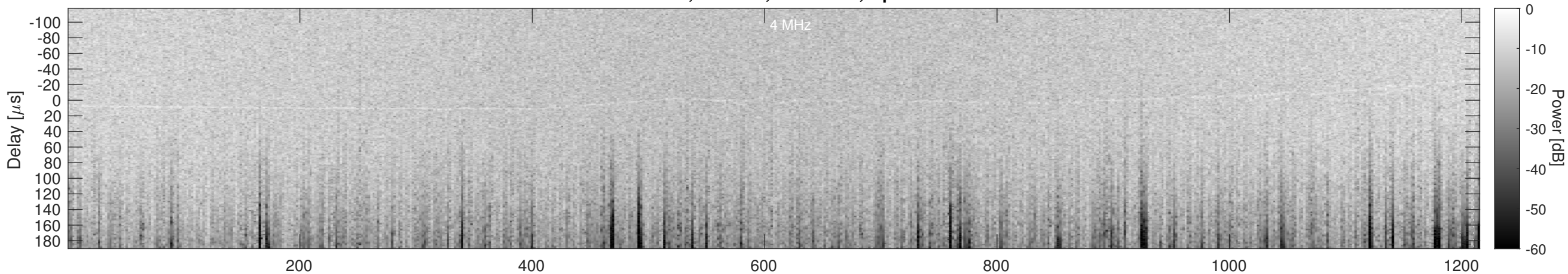
Orbit 13552, Cluttergram
