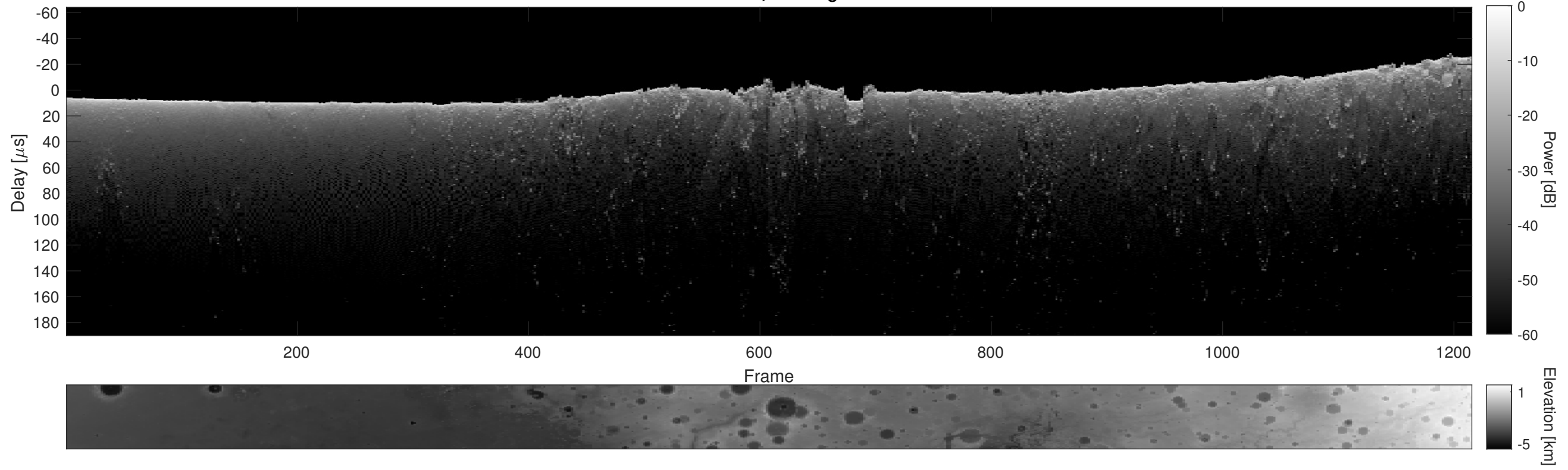
Orbit 13552, Cluttergram
