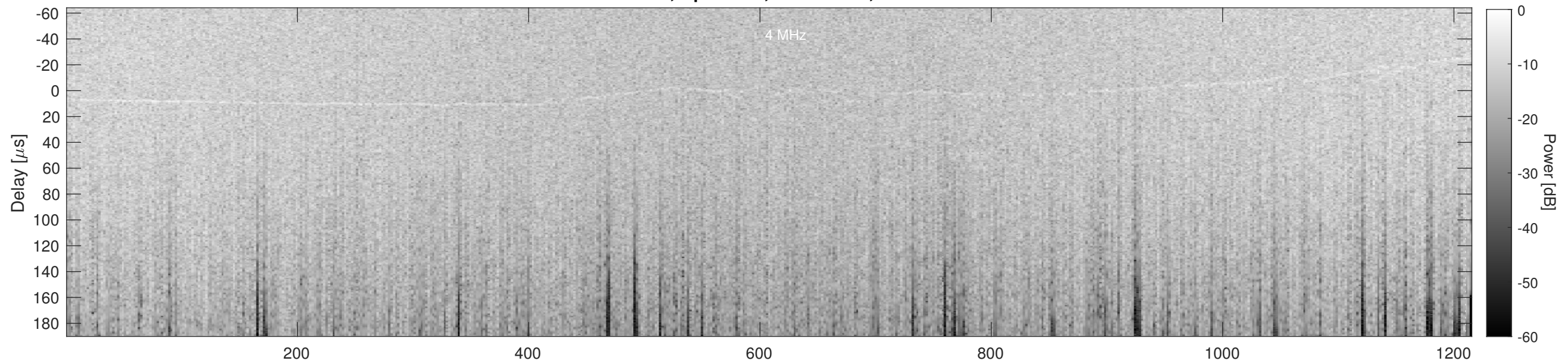
Orbit 13552, Cluttergram
