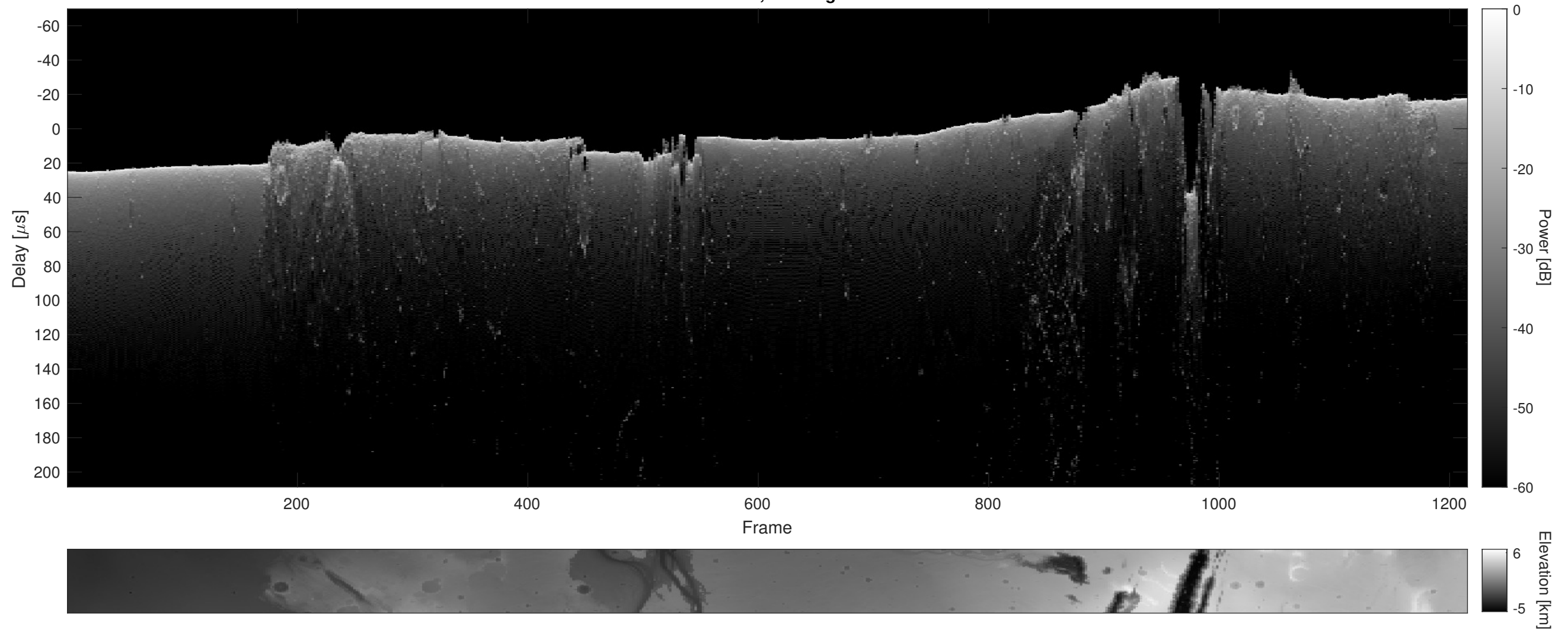
Orbit 13556, Cluttergram
