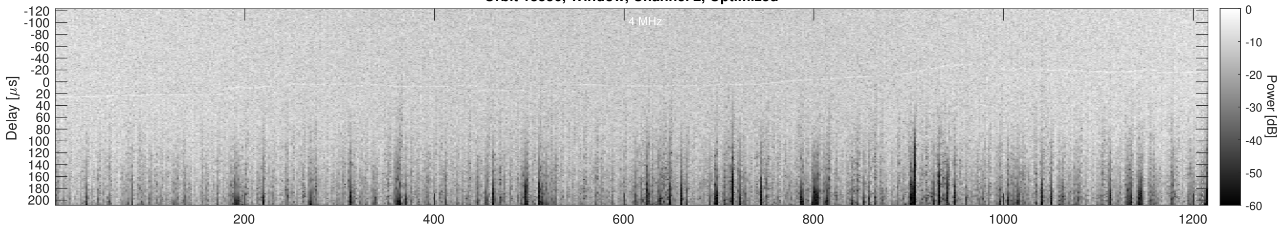
Orbit 13556, Cluttergram
