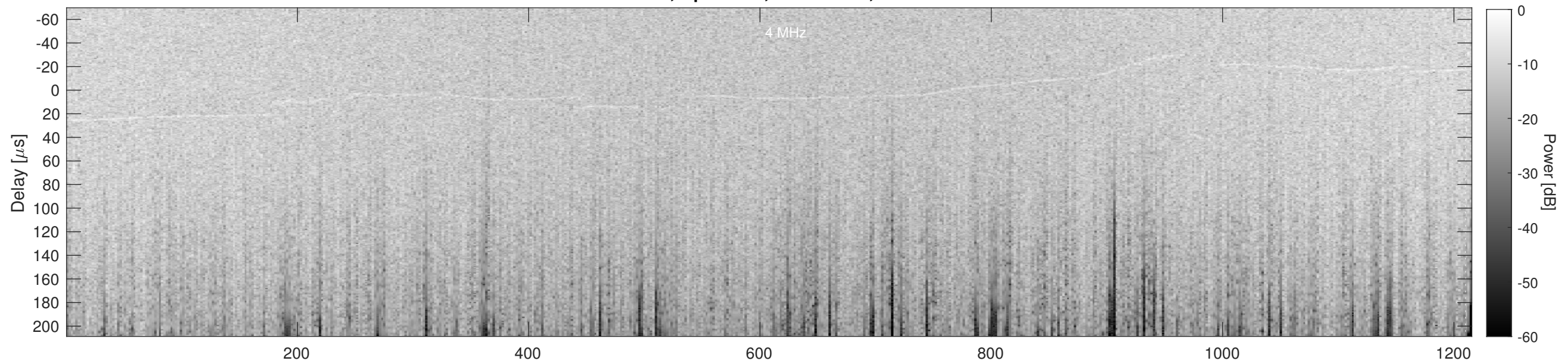
Orbit 13556, Cluttergram
