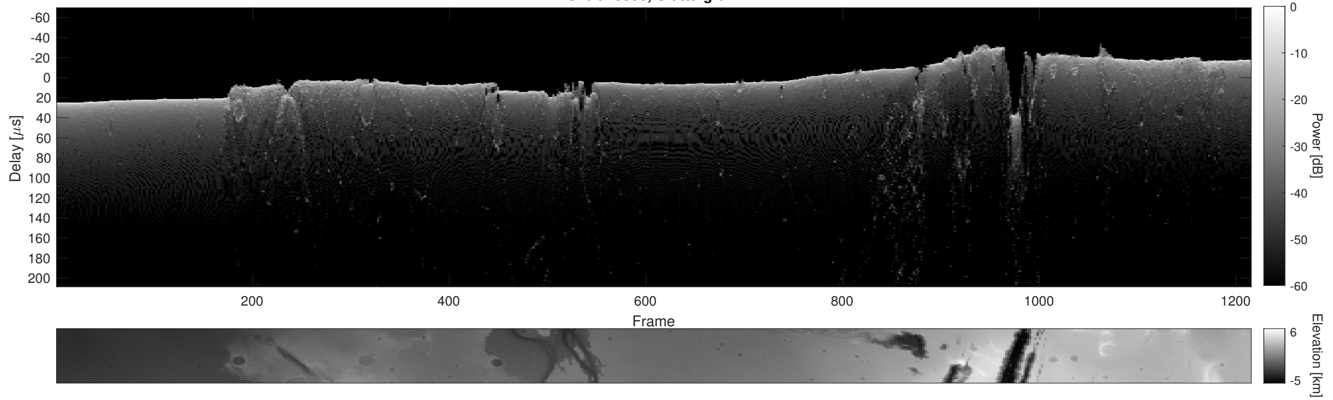
Orbit 13556, Cluttergram
