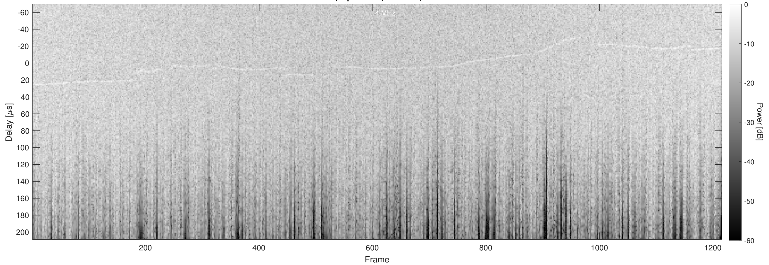
Orbit 13556, Optimized, Window, Channel 2
