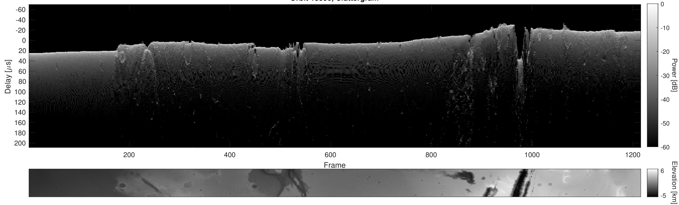
Orbit 13556, Cluttergram
