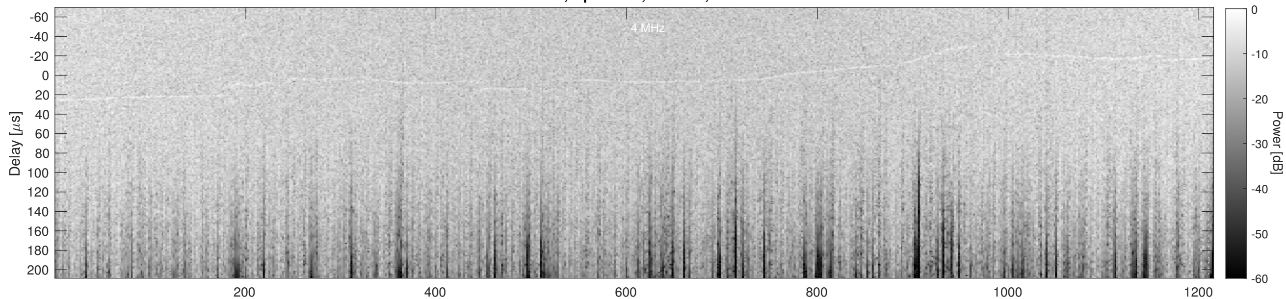
Orbit 13556, Cluttergram
