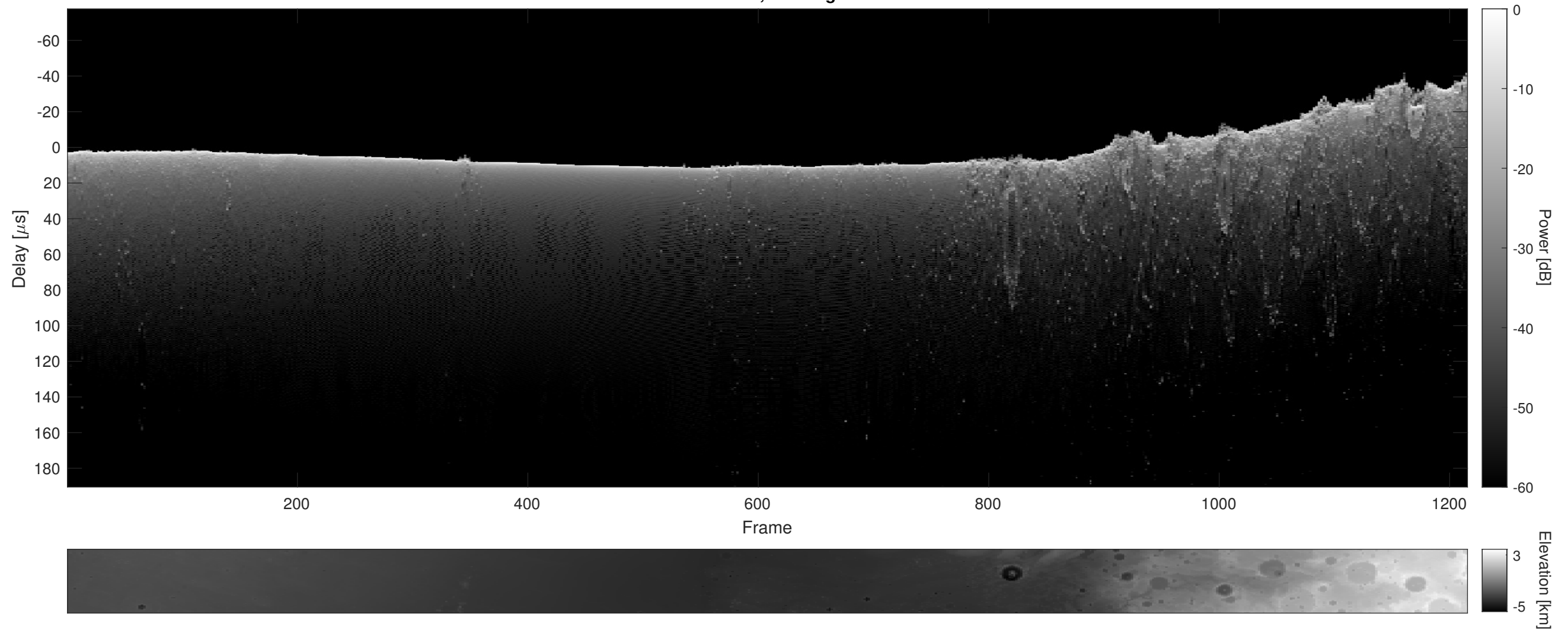
Orbit 13557, Cluttergram
