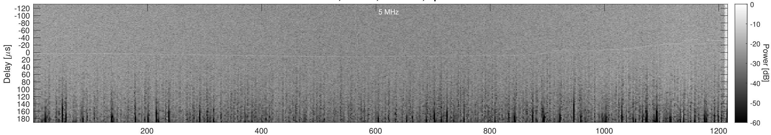
Orbit 13557, Cluttergram
