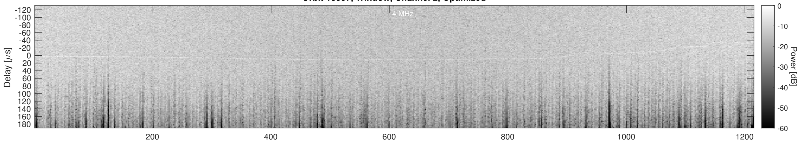
Orbit 13557, Cluttergram
