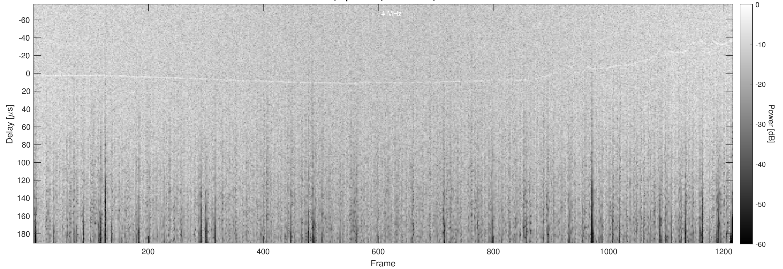
Orbit 13557, Optimized, No Window, Channel 2
