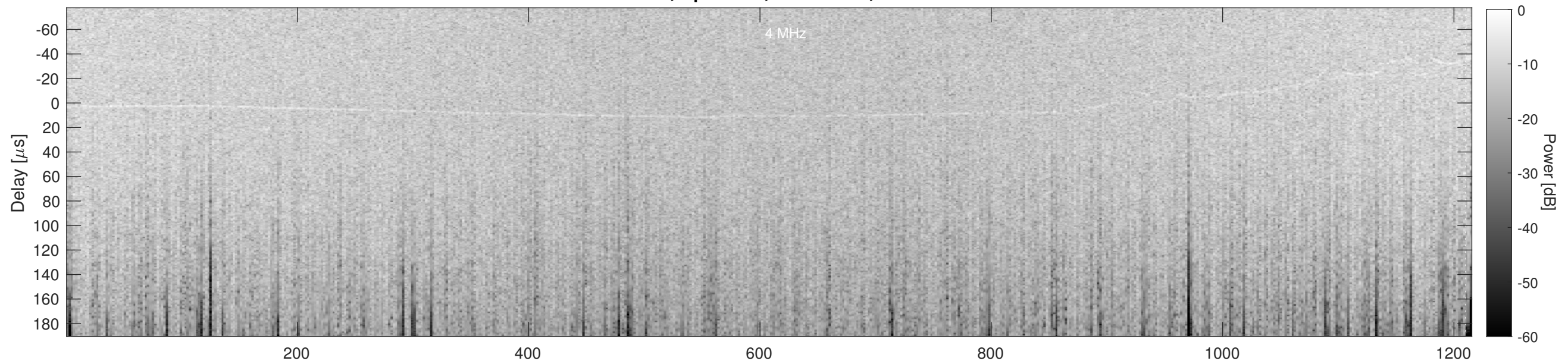
Orbit 13557, Cluttergram
