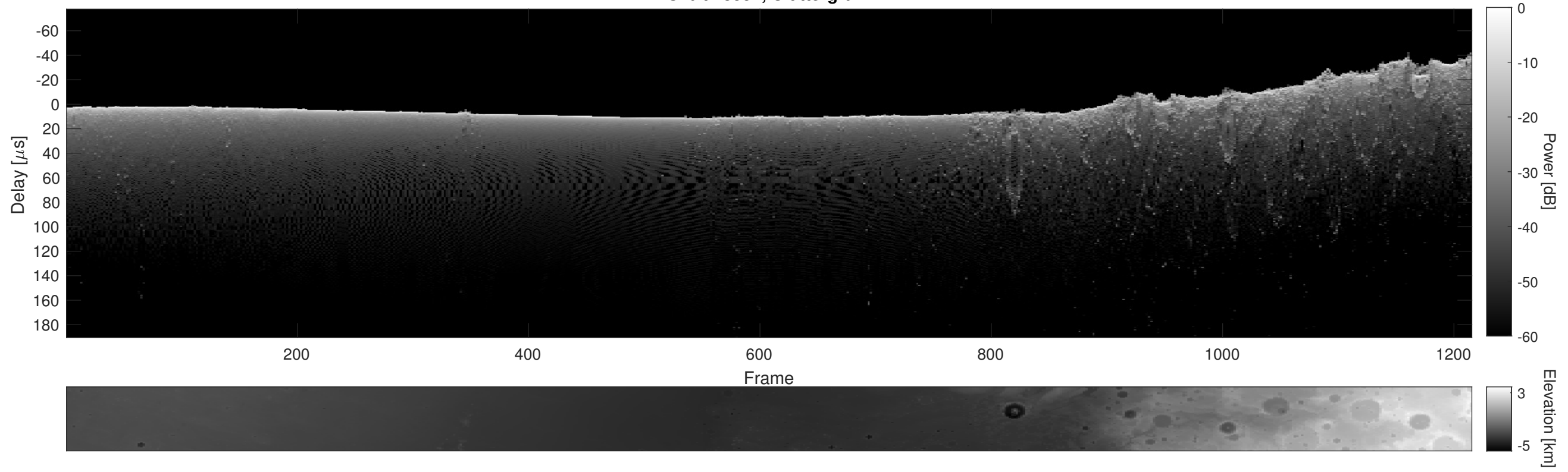
Orbit 13557, Cluttergram
