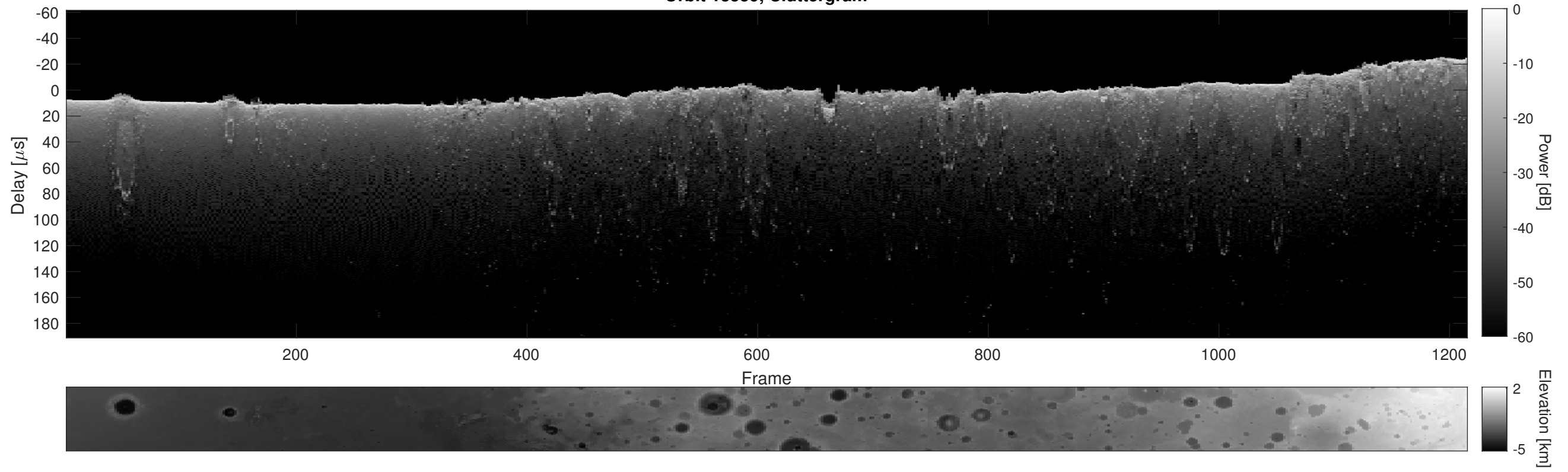
Orbit 13559, Cluttergram
