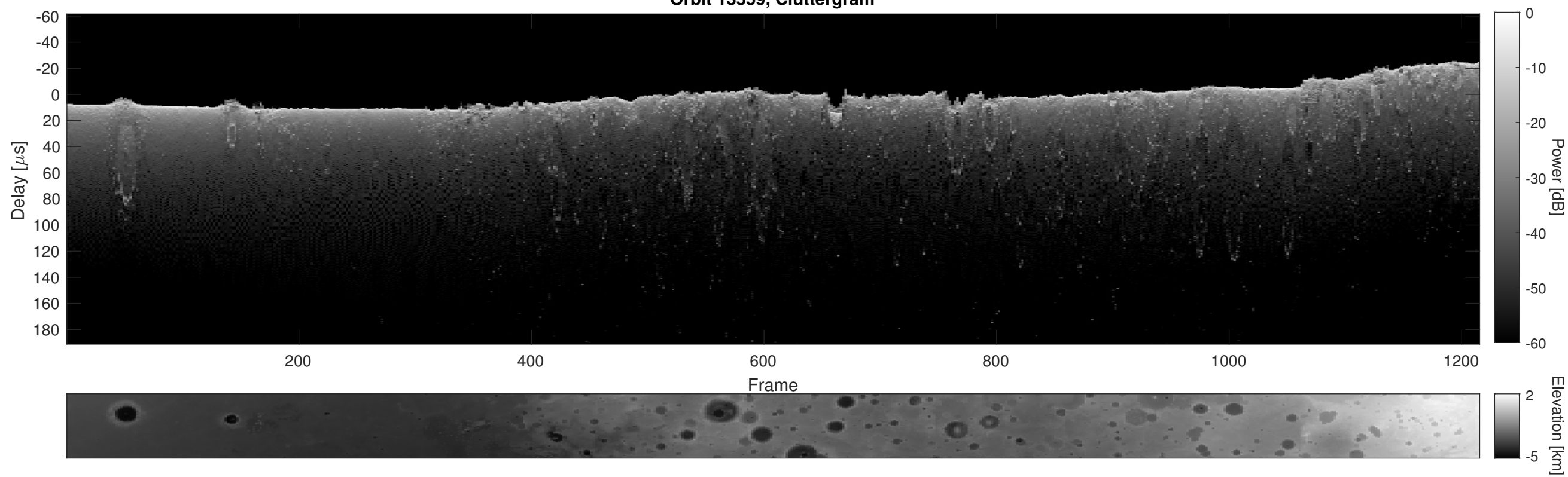
Orbit 13559, Cluttergram
