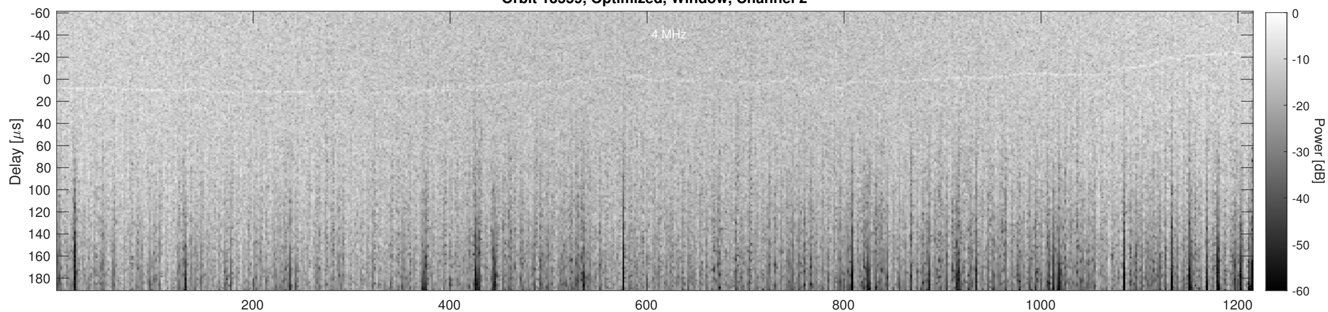
Orbit 13559, Cluttergram
