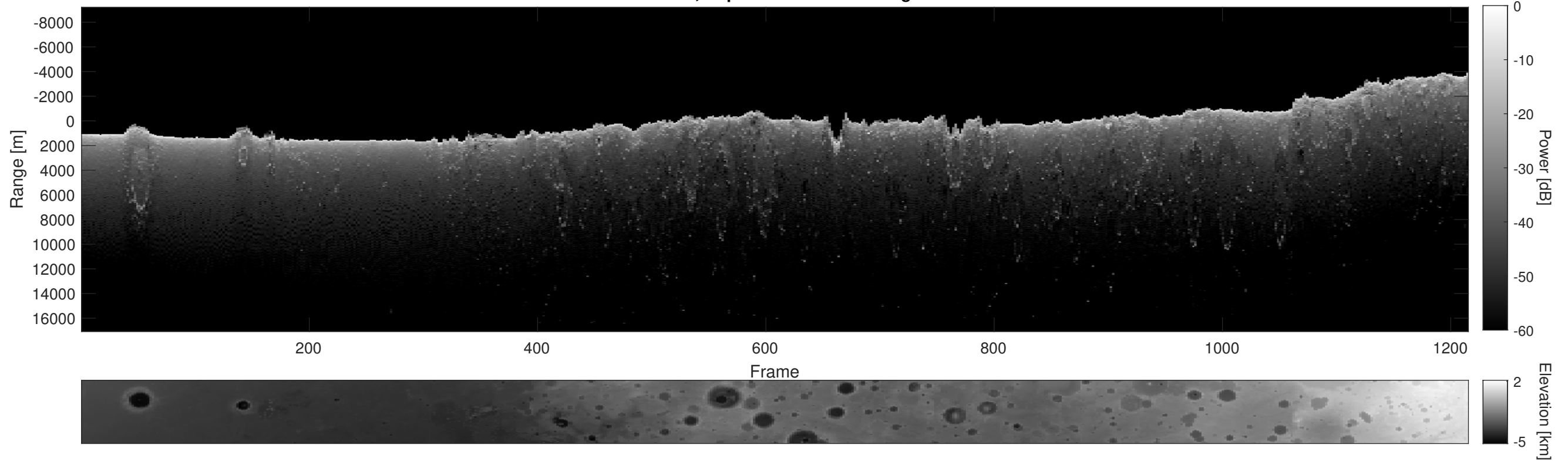
Orbit 13559, Depth-Corrected Cluttergram
