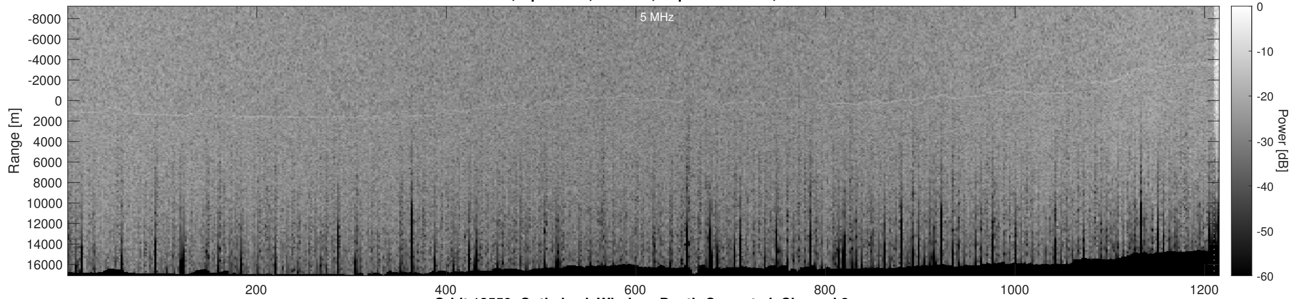
Orbit 13559, Optimized, Window, Depth-Corrected, Channel 2
