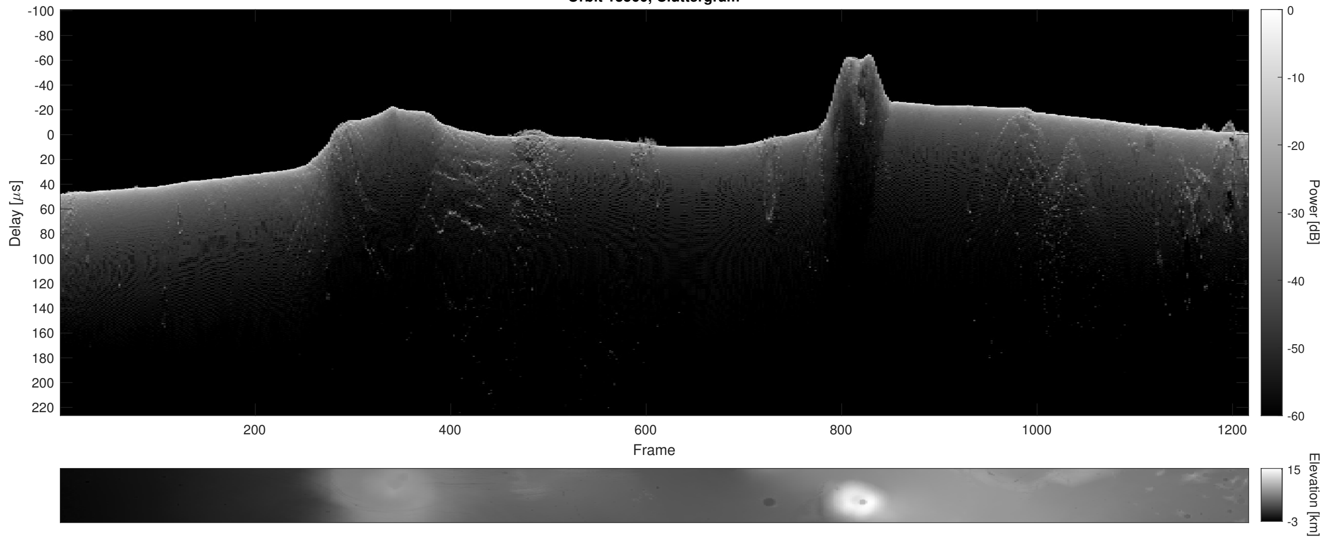
Orbit 13560, Cluttergram
