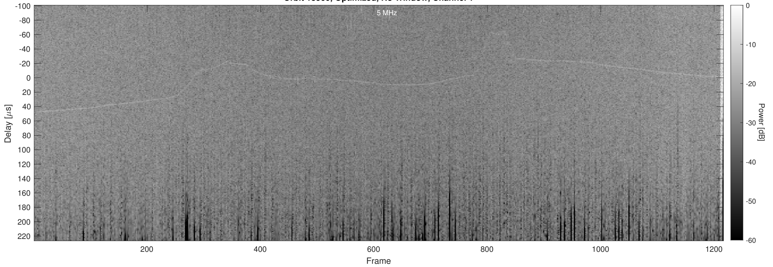
Orbit 13560, Optimized, No Window, Channel 2
