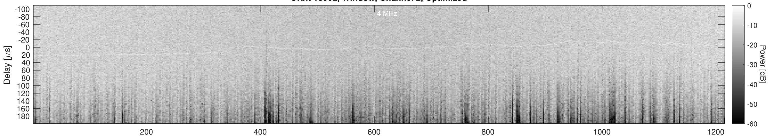
Orbit 13562, Cluttergram
