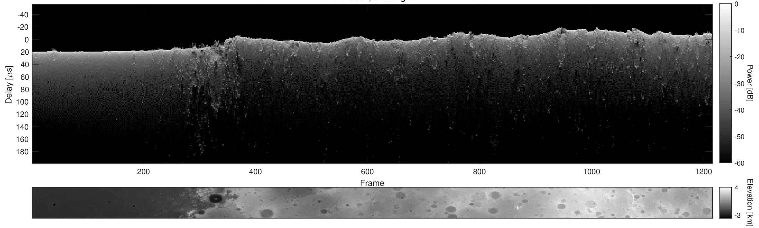
Orbit 13562, Cluttergram
