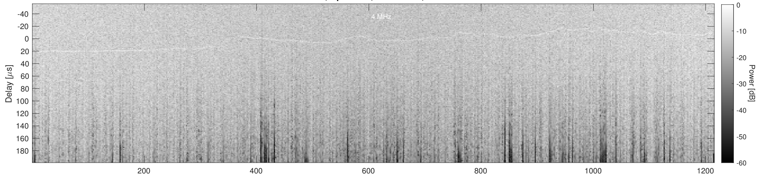
Orbit 13562, Cluttergram
