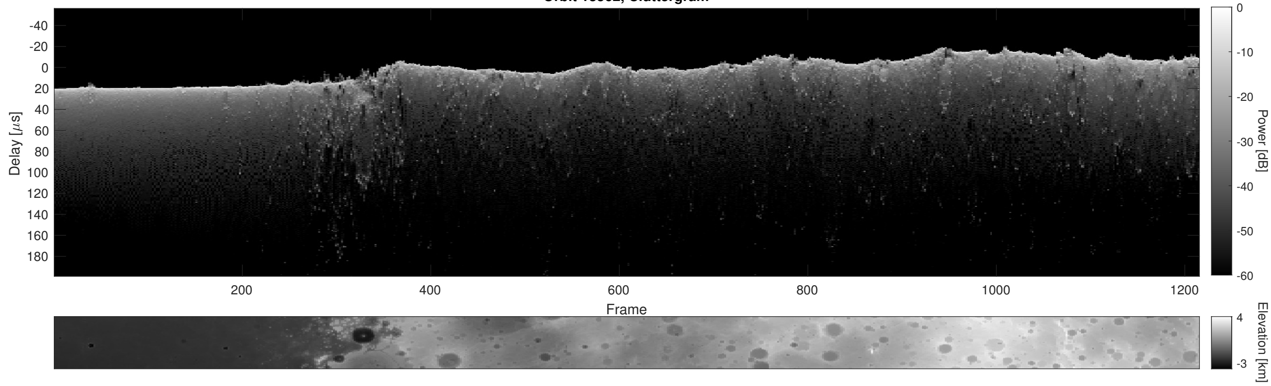
Orbit 13562, Cluttergram
