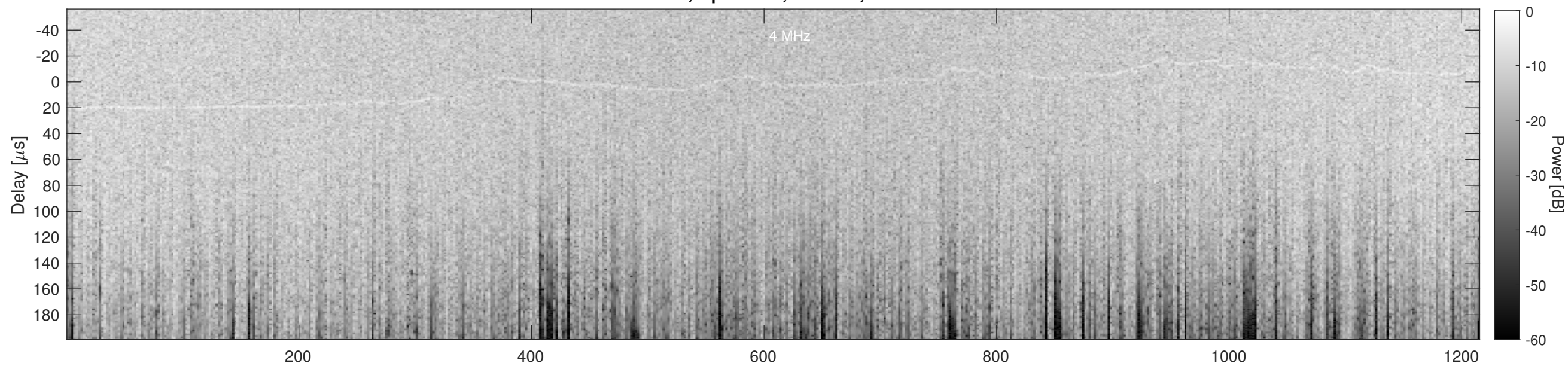
Orbit 13562, Cluttergram
