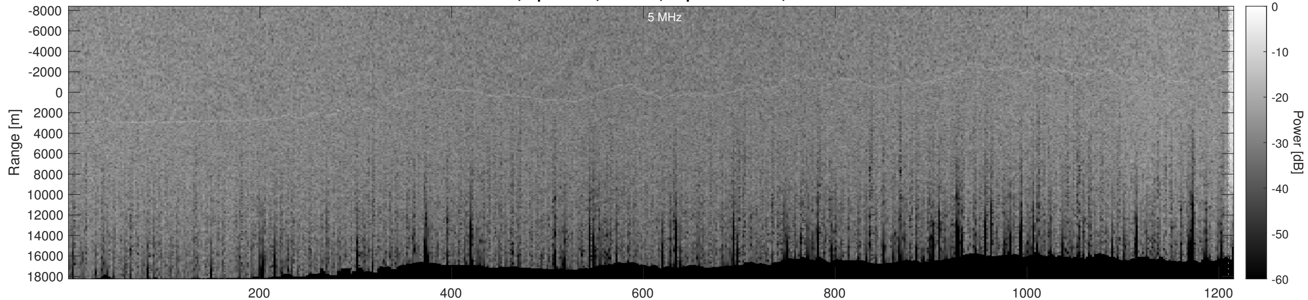
Orbit 13562, Optimized, Window, Depth-Corrected, Channel 2
