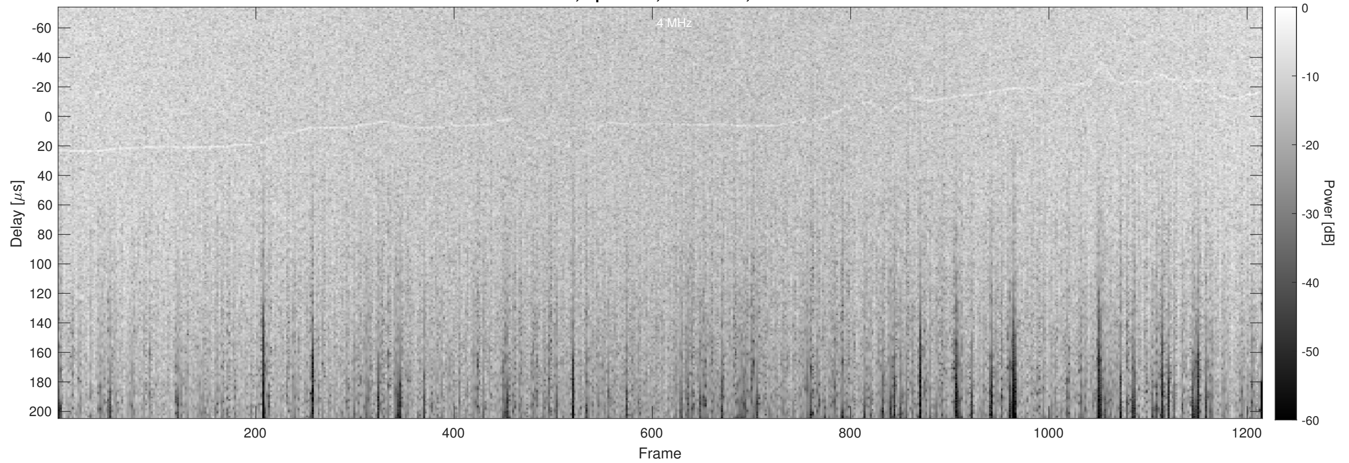
Orbit 13563, Optimized, No Window, Channel 2
