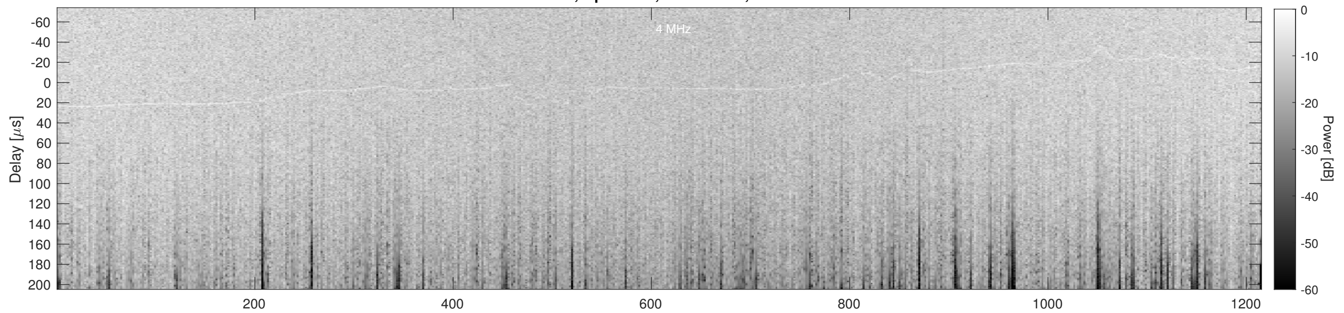
Orbit 13563, Cluttergram
