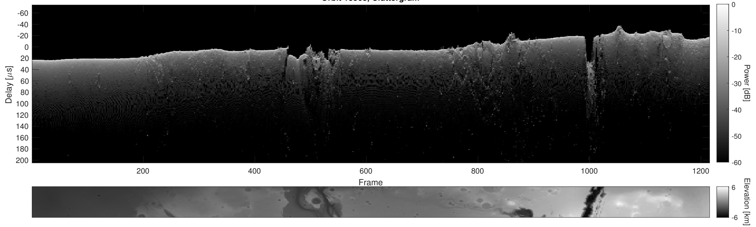
Orbit 13563, Cluttergram
