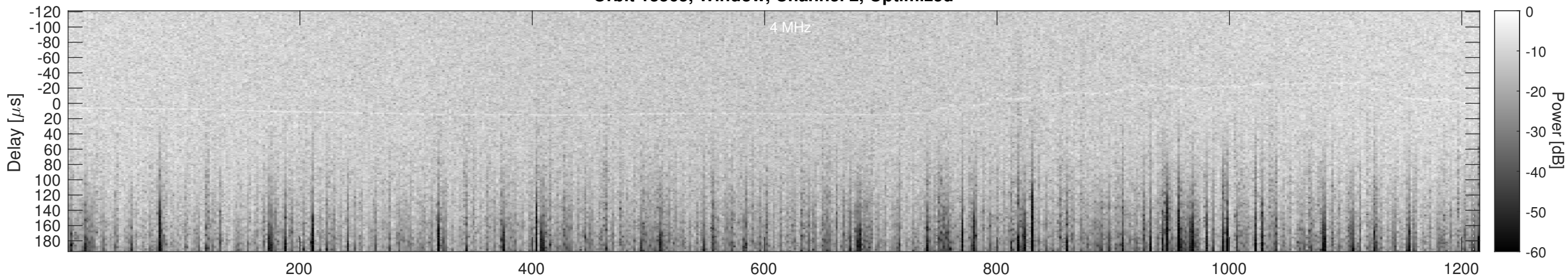
Orbit 13565, Cluttergram
