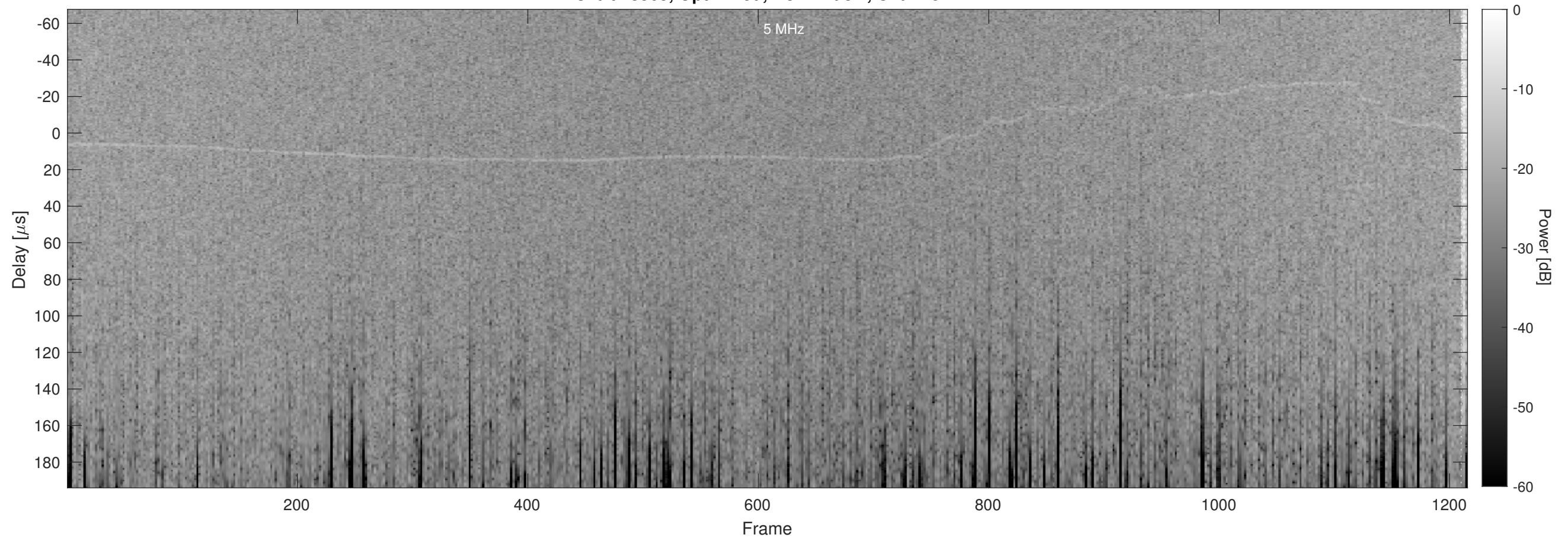
Orbit 13565, Optimized, No Window, Channel 2
