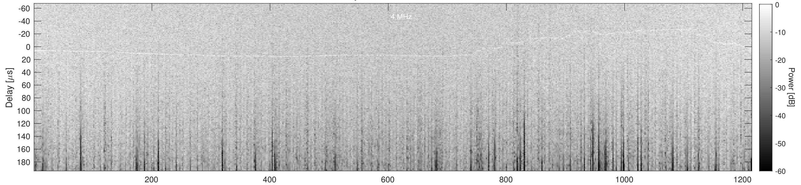
Orbit 13565, Cluttergram
