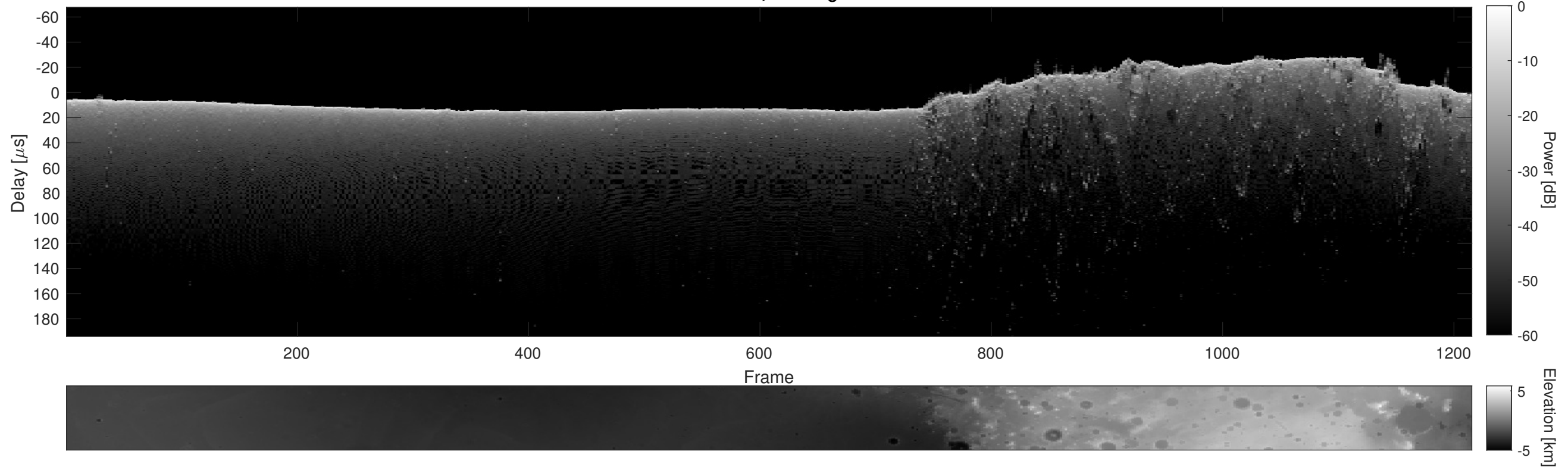
Orbit 13565, Cluttergram
