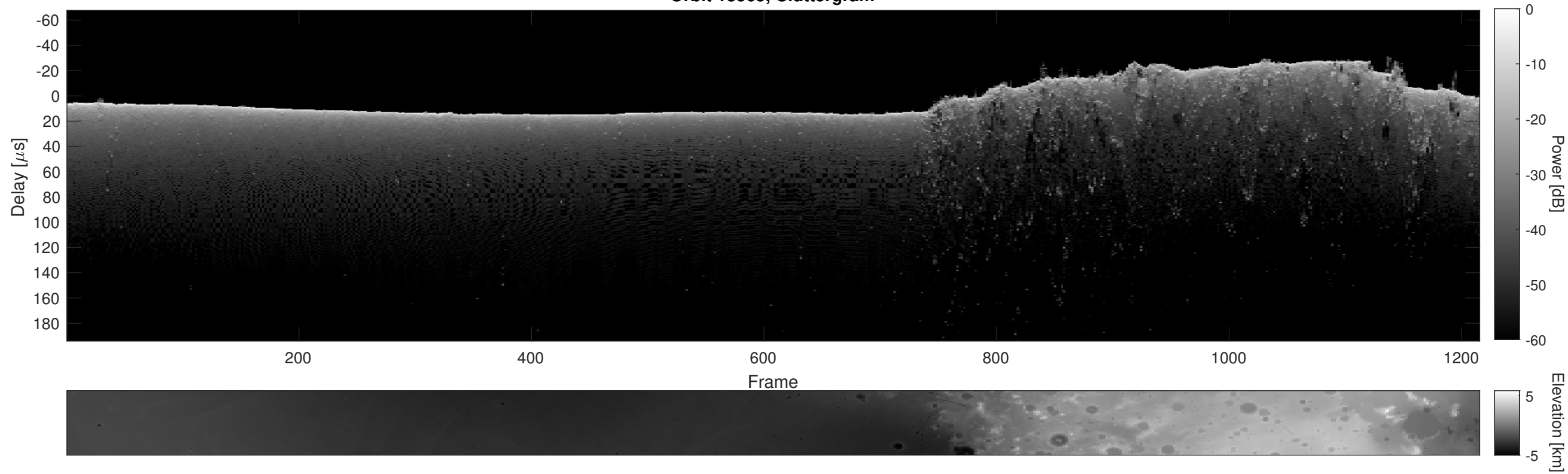
Orbit 13565, Cluttergram
