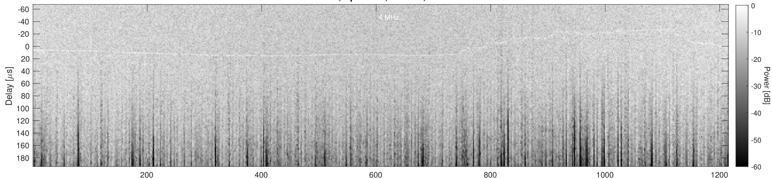
Orbit 13565, Cluttergram
