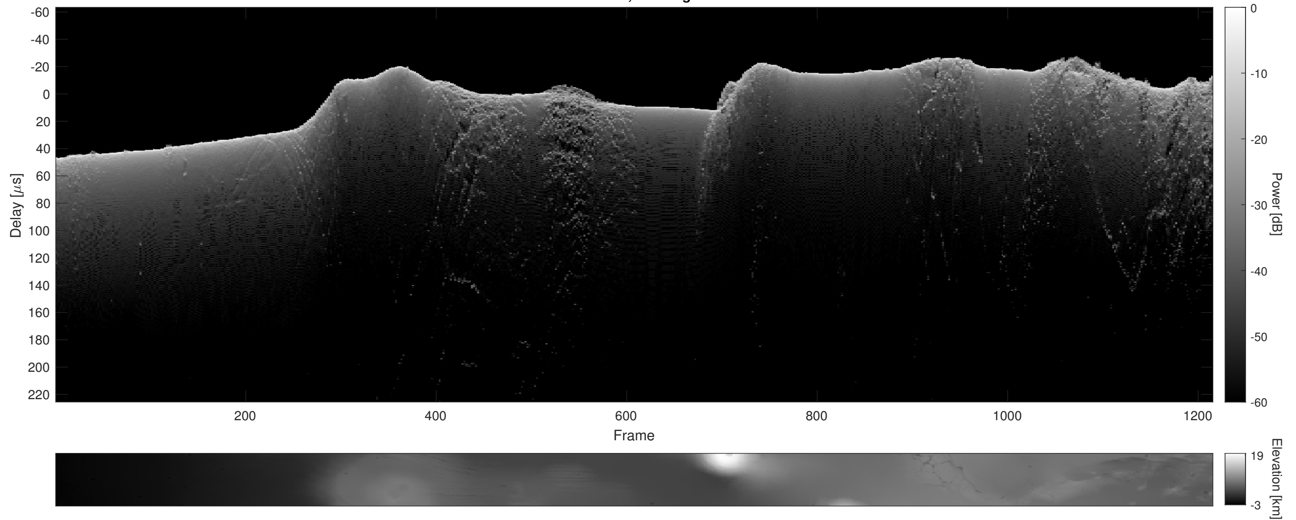
Orbit 13567, Cluttergram
