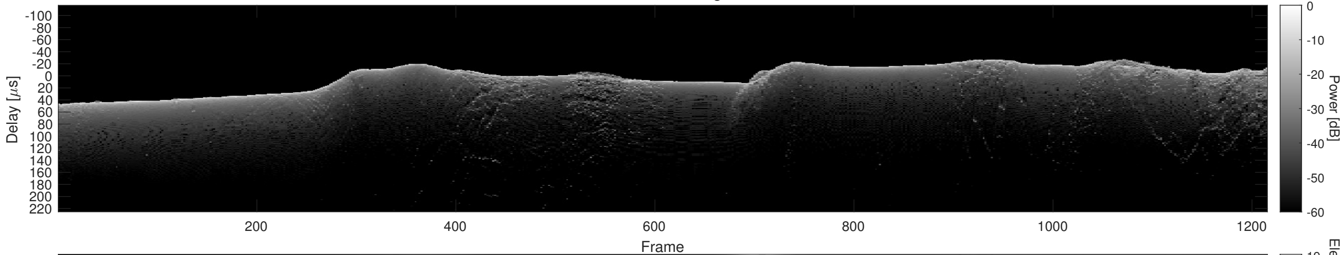
Orbit 13567, Cluttergram
