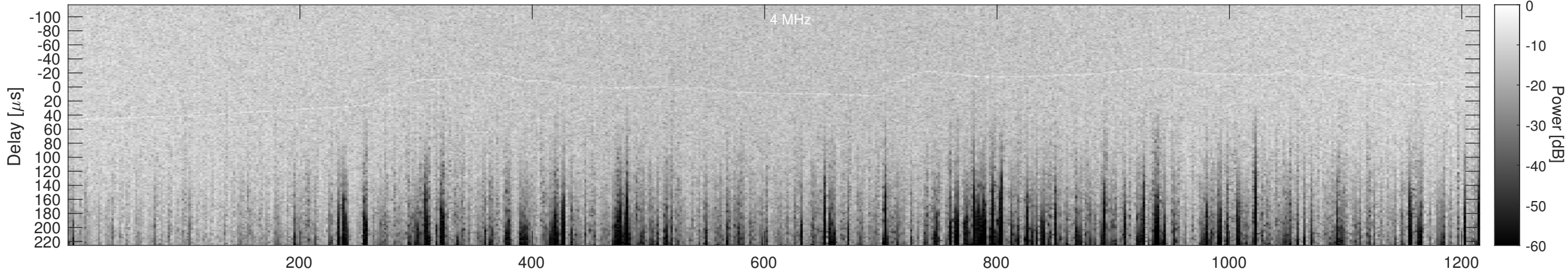
Orbit 13567, Cluttergram
