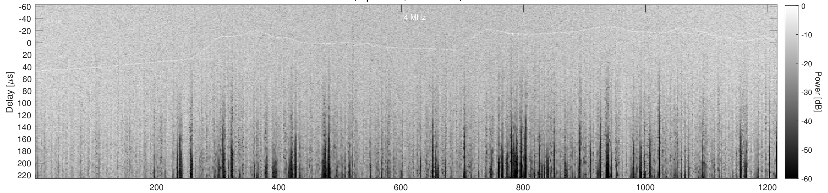
Orbit 13567, Cluttergram
