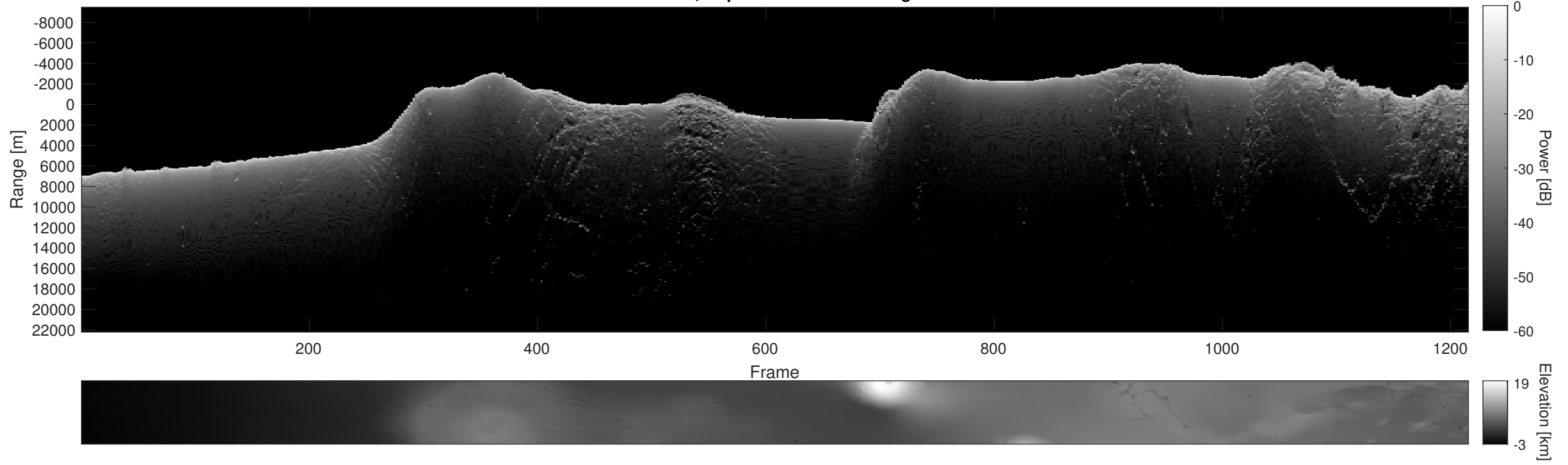
Orbit 13567, Depth-Corrected Cluttergram
