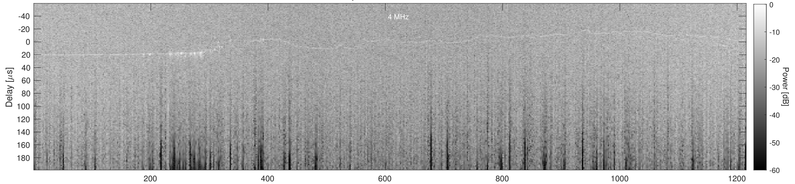
Orbit 13569, Cluttergram
