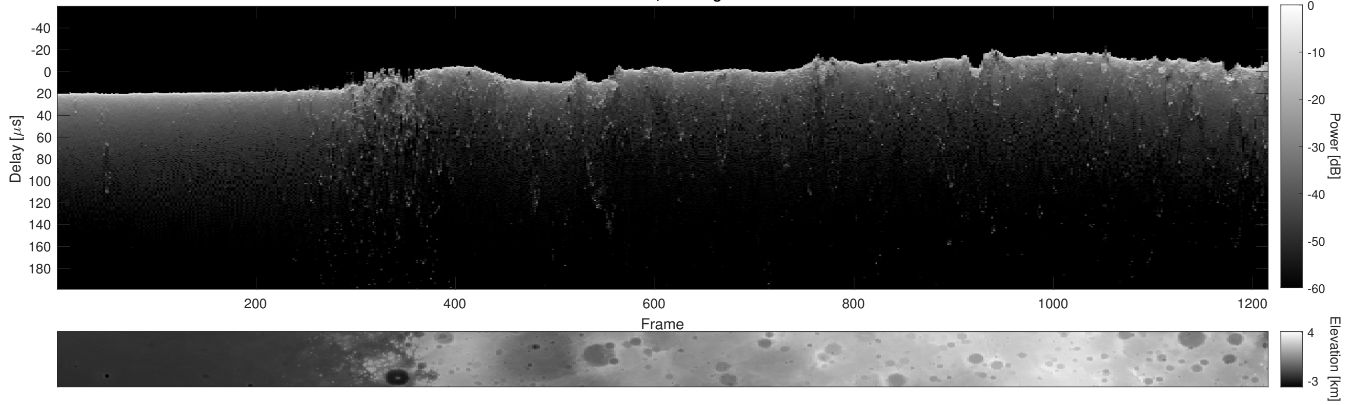
Orbit 13569, Cluttergram
